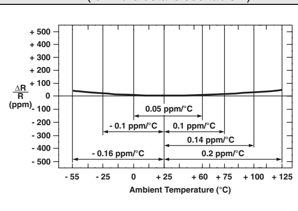
FIGURE 4 - TYPICAL TCR CURVE Z-FOIL (for more details see table 1)
