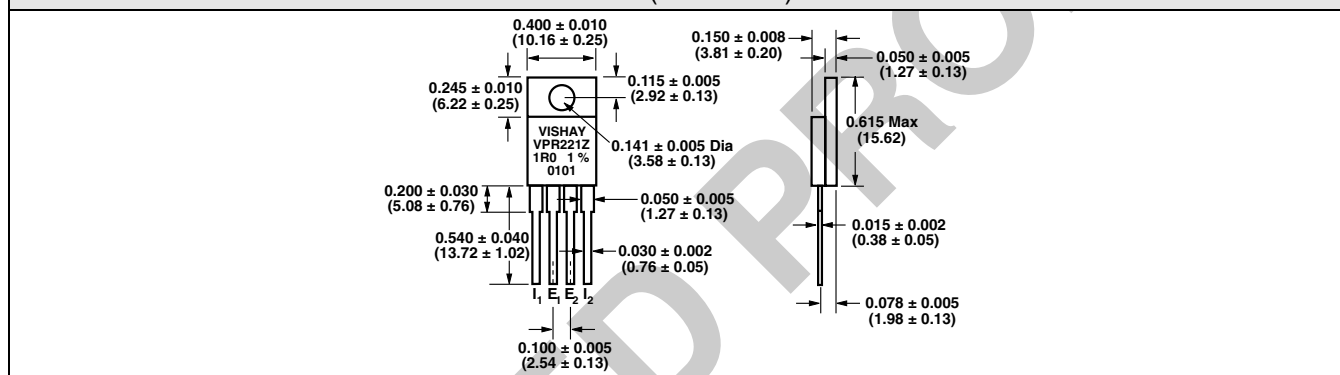
FIGURE 4 - VPR221Z DIMENSIONS in inches (millimeters)
