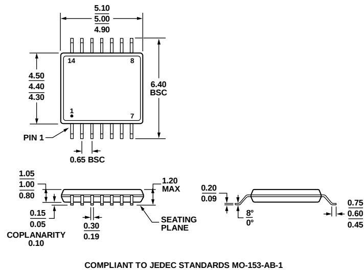
Figure 16. 14-Lead Thin Shrink Small Outline Package (RU-14) Dimensions shown in millimeters
