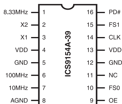
16-Pin SOIC
