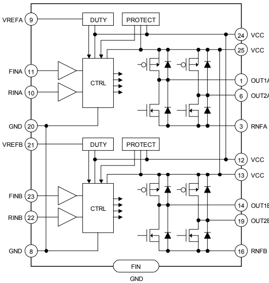
Fig.31 BD6215FP / BD6216FP
