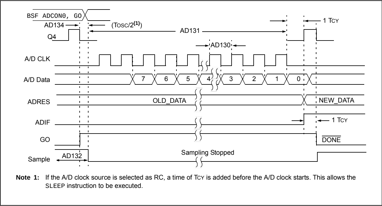
FIGURE 30-12: PIC16(L)F1938/39 A/D CONVERSION TIMING (NORMAL MODE)
