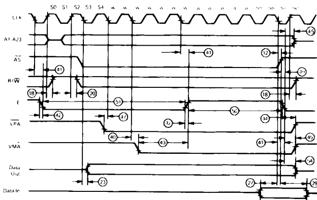
Figure 8.9 : TS68000 to 6800 Peripheral Timing Diagram – Best Case.
