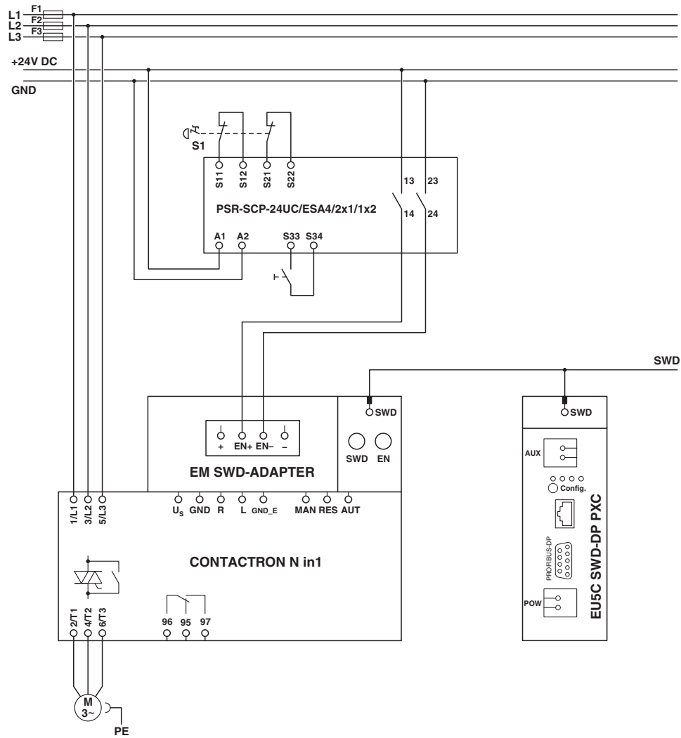
Circuit diagram
