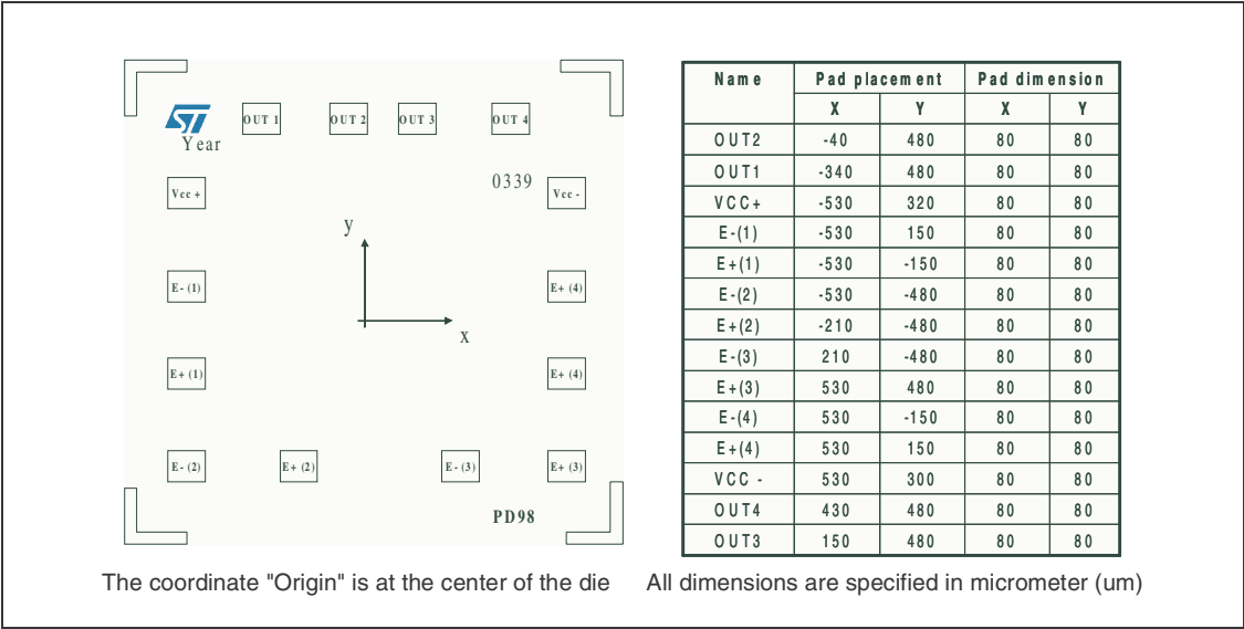
Figure 2. Pad locations
