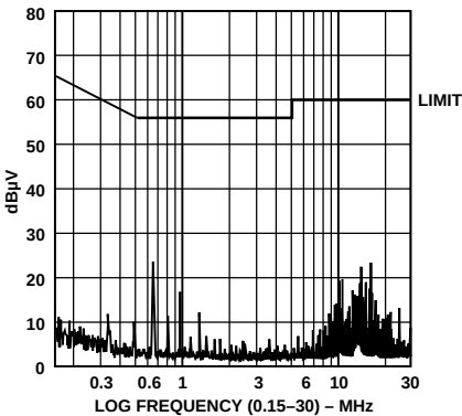
Figure 24. Conducted Emissions
