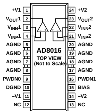
Figure 1. 24-Lead SOIC_W_BAT (RB-24)
