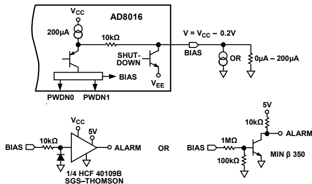
Figure 44. Shutdown and Alarm Circuit
