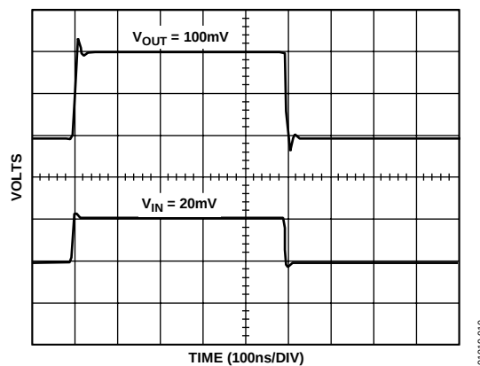
Figure 9. 100 mV Step Response; G = +5 , V_S = \pm 12\text{ V} , R_L = 25\ \Omega , Single-Ended
