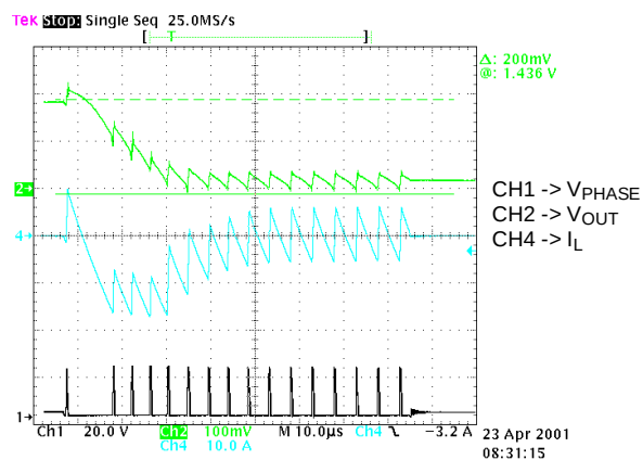
Figure 2. Dynamic Output Voltage Transition 1.55V -> 1.35V
