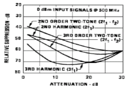
Distortion Products
