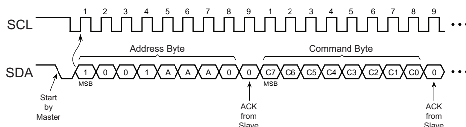
Figure 9-1. Command Loading
