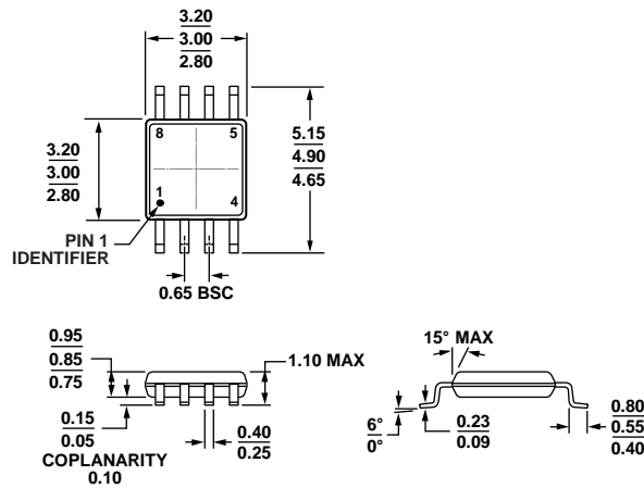
COMPLIANT TO JEDEC STANDARDS MO-187-AA Figure 62. 8-Lead Mini Small Outline Package [MSOP] (RM-8)
