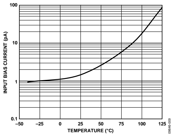
Figure 17. Input Bias Current vs. Temperature, V_{SY} = \pm 5V
