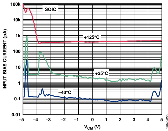
Figure 16. Input Bias Current vs. Common-Mode Input Voltage ( V_{CM} ), V_{SY} = \pm 5V, R_L = \infty
