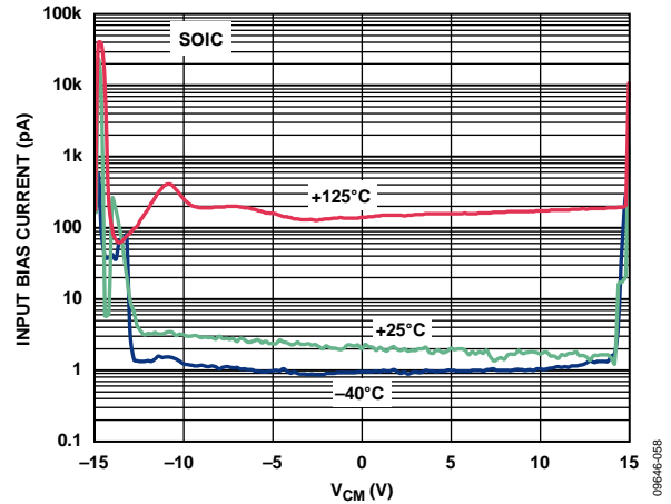
Figure 19. Input Bias Current vs. Common-Mode Input Voltage ( V_{CM} ), V_{SY} = \pm 15V, R_L = \infty
