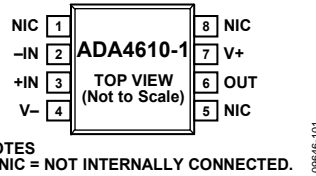
Figure 2. ADA4610-1 Pin Configuration, 8-Lead SOIC (R Suffix)
