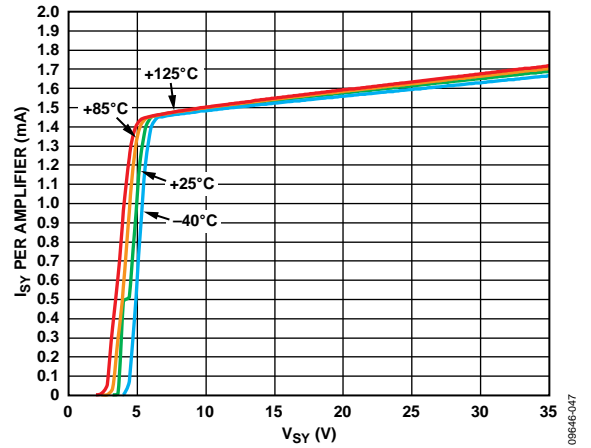
Figure 52. Supply Current ( I_{SV} ) per Amplifier vs. Supply Voltage ( V_{SY} ) at Various Temperatures
