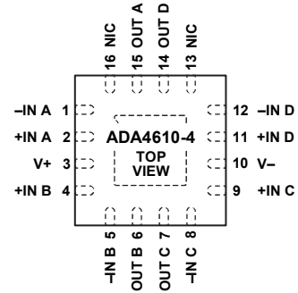
Figure 8. ADA4610-4 Pin Configuration, 16-Lead LFCSP (CP Suffix)
