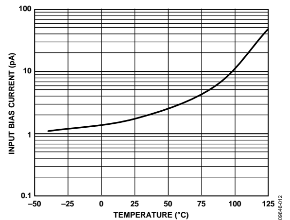
Figure 20. Input Bias Current vs. Temperature, V_{SY} = \pm 15V
