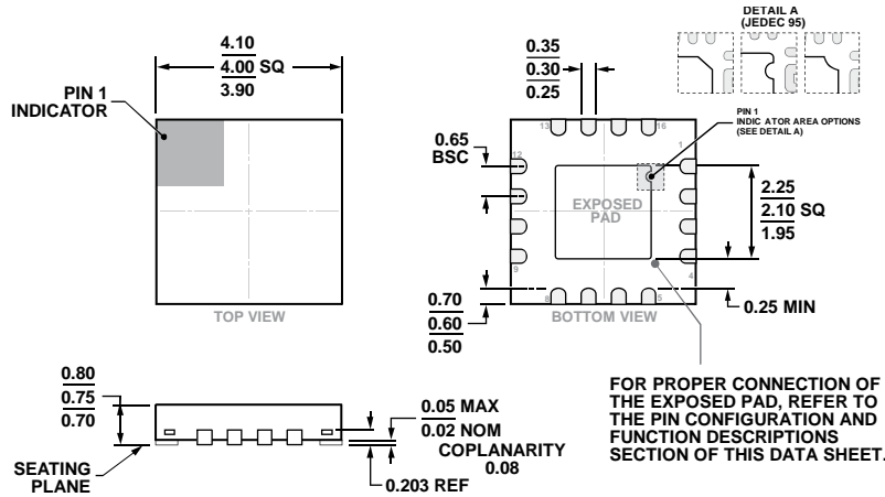
Figure 66. 16-Lead Lead Frame Chip Scale Package [LFCSP] 4 mm x 4 mm Body and 0.75 mm Package Height (CP-16-23)
