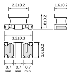
LQH3N Type
