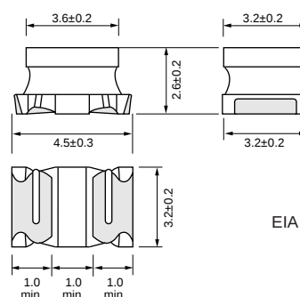
LQH4N/LQN4N Type
