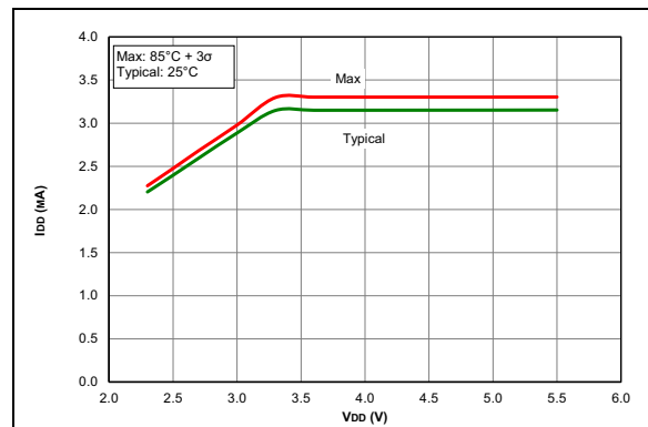
FIGURE 38-6: I_{DD} , HFINTOSC Mode, F_{OSC} = 32 MHz, PIC16F15325/45 Only.
