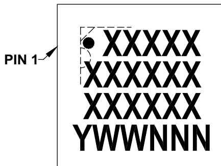
16-Lead QFN/VQFN (4x4x0.9 mm)
