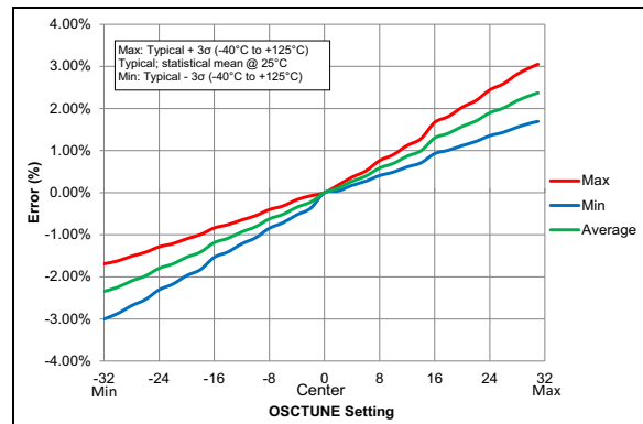
FIGURE 38-105: OSCTUNE Center Frequency, PIC16LF15325/45 Only.
