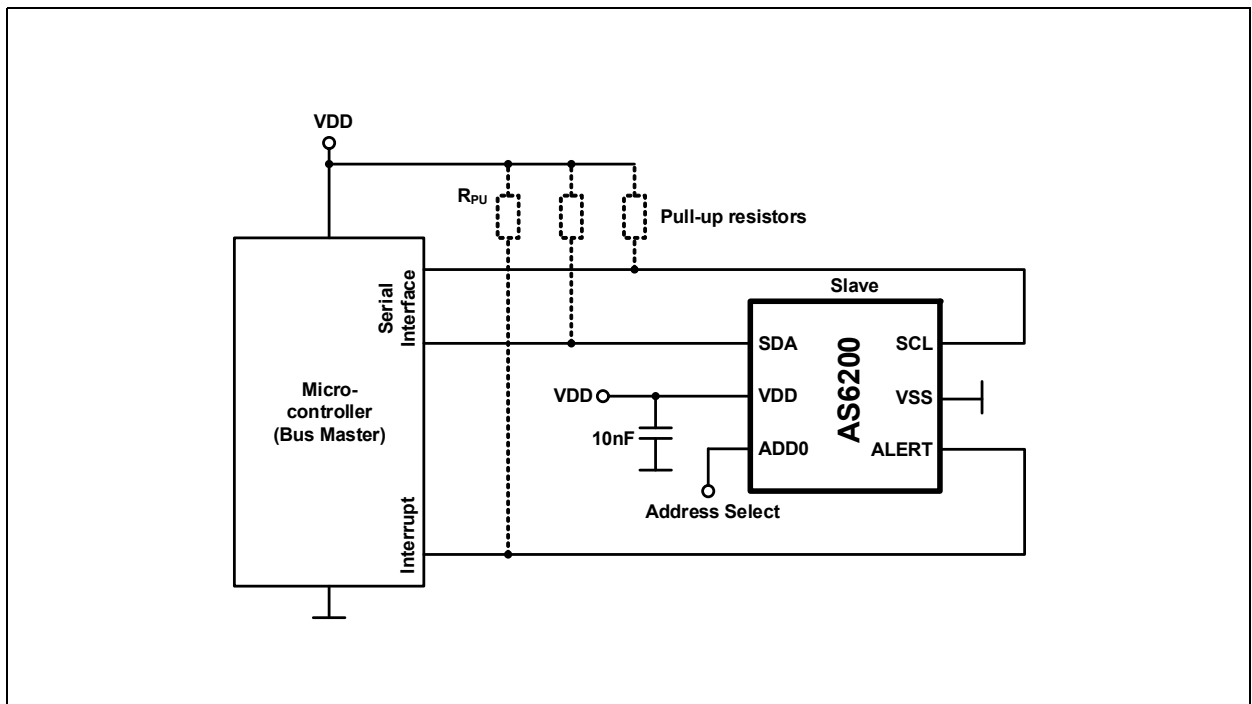
Figure 2: Typical Application Environment of the AS6200 Temperature Sensor
