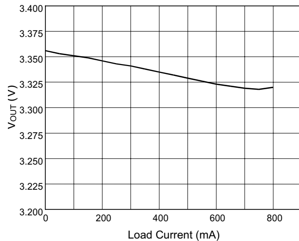
Fig. 16 Load Regulation
