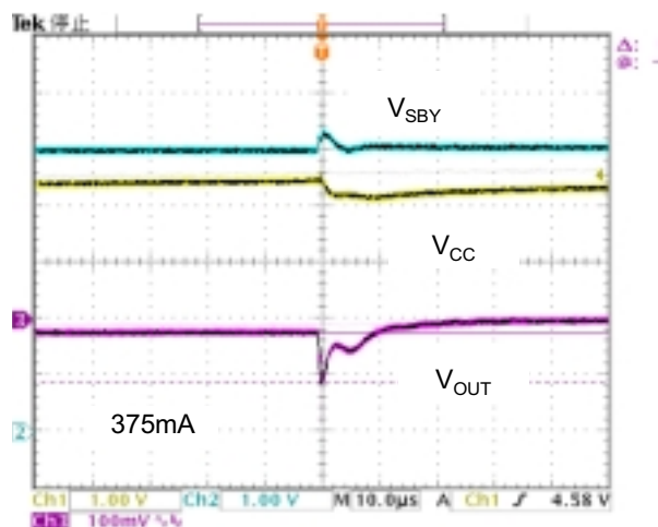
Fig. 7 V_{CC} Power Up ( V_{SBY} = 5V )
