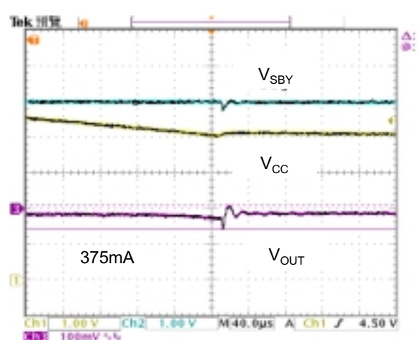
Fig. 8 V_{CC} Power down ( V_{SBY} = 5V )
