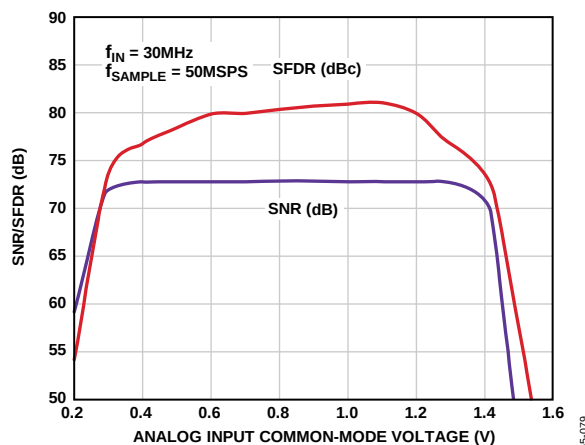
Figure 37. SNR/SFDR vs. Common-Mode Voltage, f_{IN} = 30 \text{ MHz} , f_{SAMPLE} = 50 \text{ MSPS}
