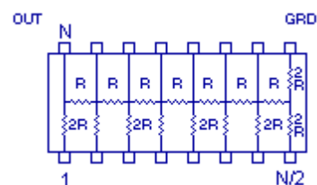
R/2R Ladder (Schematic 7)
