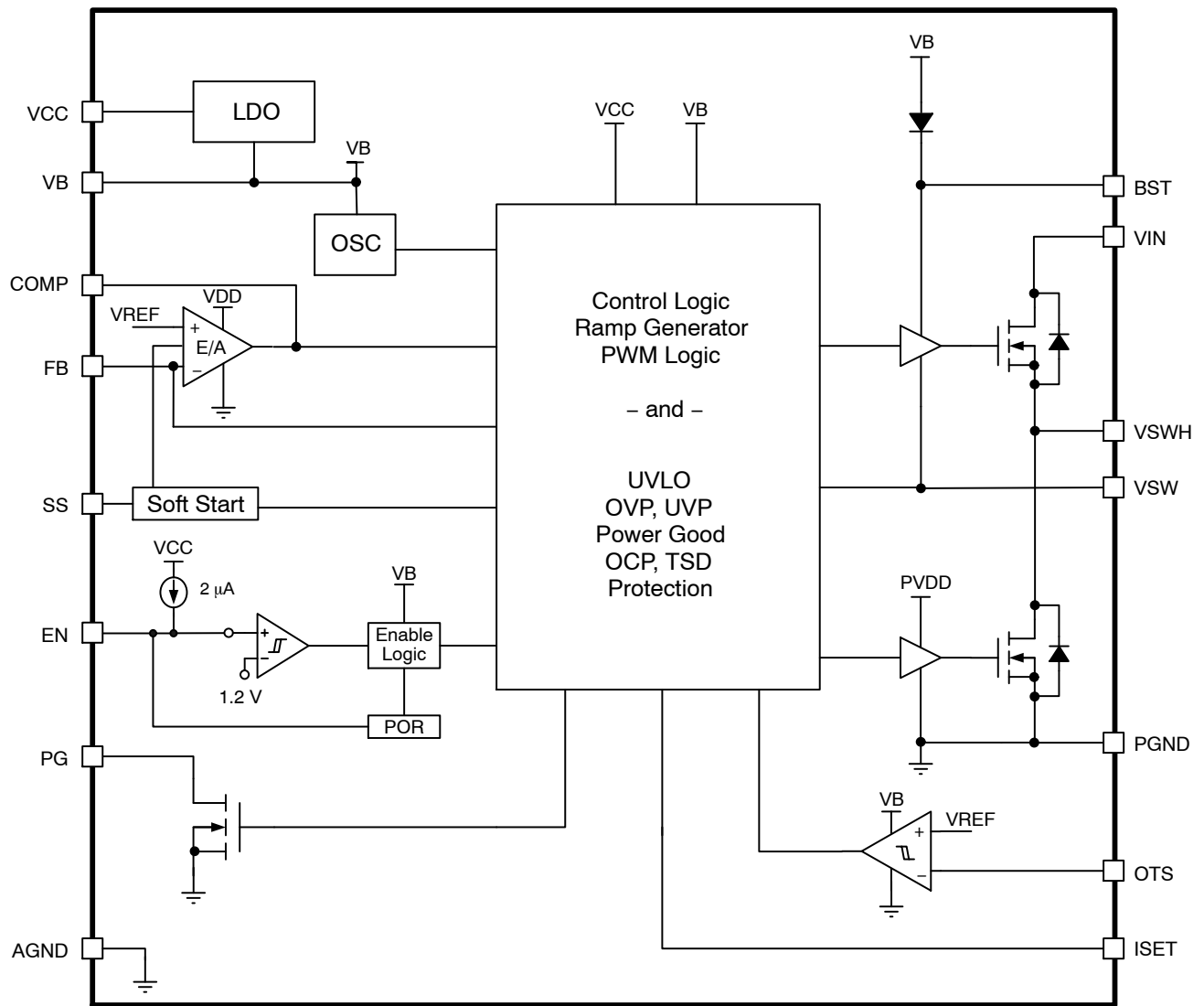
Figure 1. NCP3231B Block Diagram
