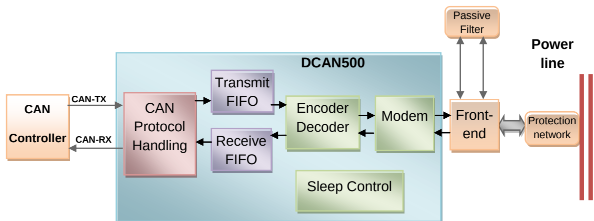
Figure 2 - DCAN500 Block Diagram
