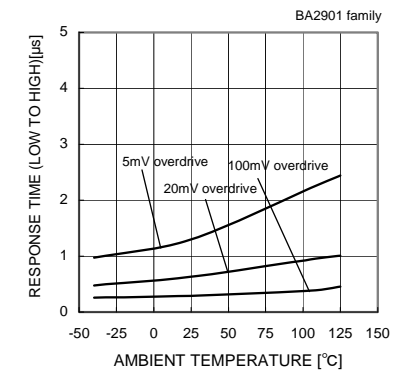
Fig.107 Response Time (Low to High) - Ambient Temperature (VCC=5[V],VRL=5[V],RL=5.1[kΩ])
