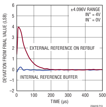
Figure 13. Burst Conversion Response of the LTC2344-16, f_{\text{SMPL}} = 400\text{ksps}
