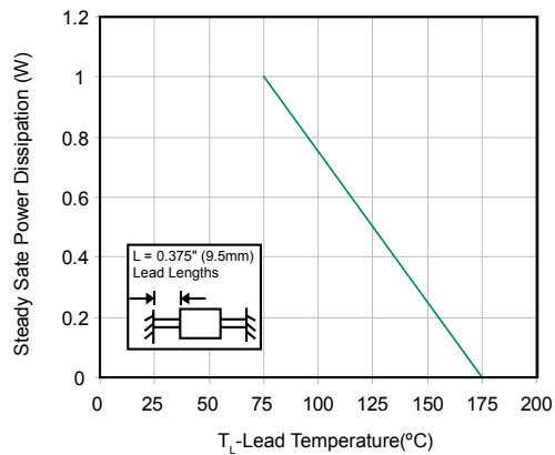
Figure 5 - Steady Pulse Derating Curve
