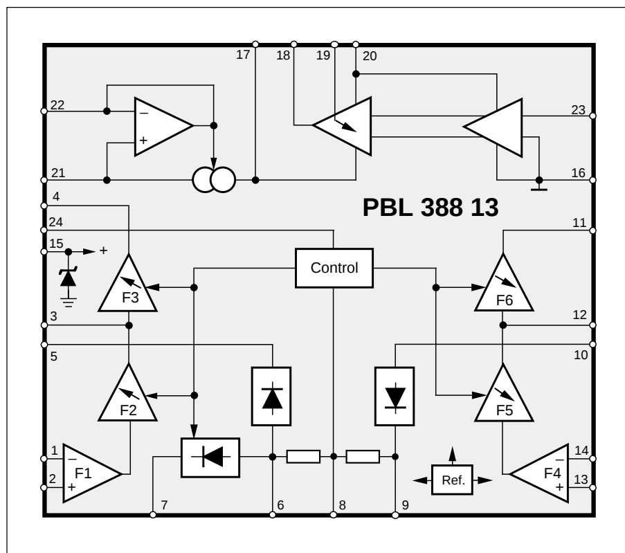
Figure 1. Block diagram.
