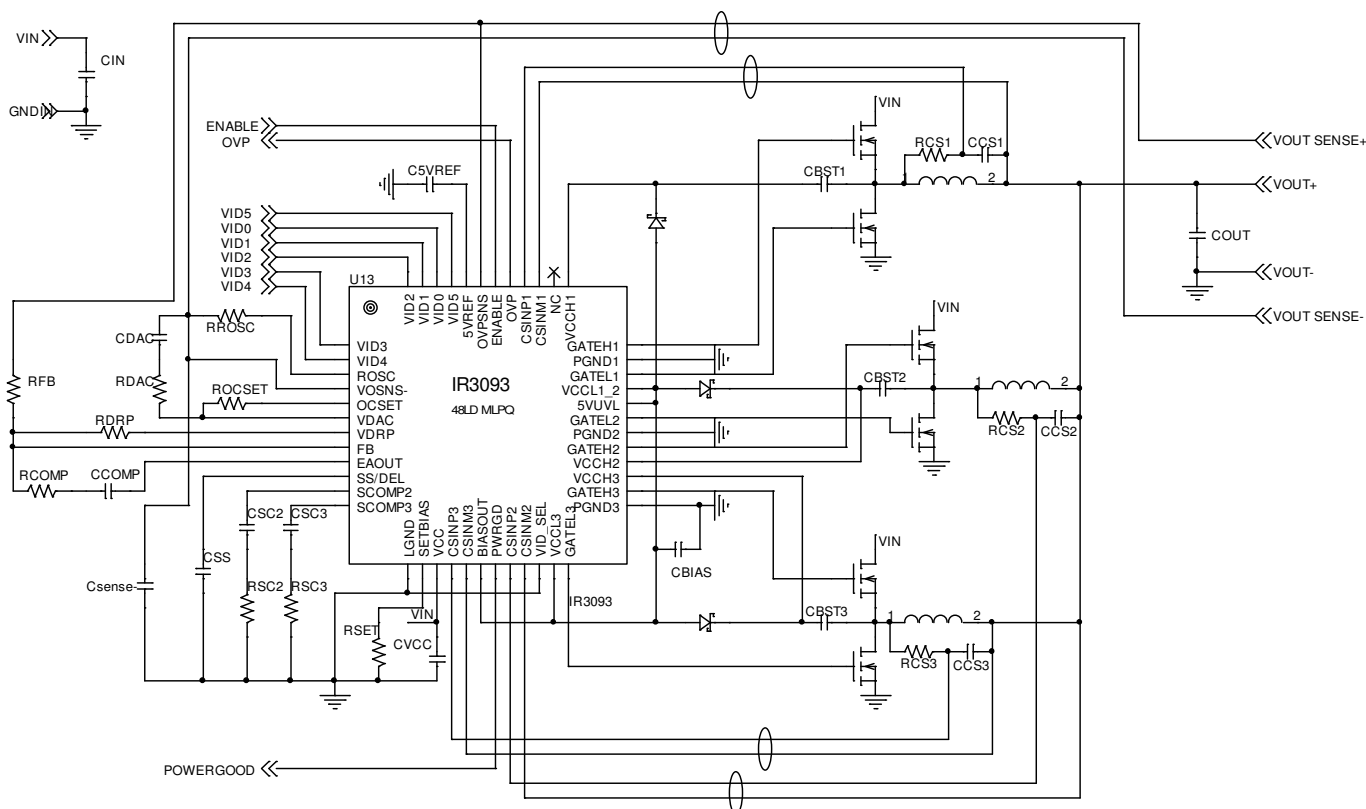
Figure 6 – System Diagram
