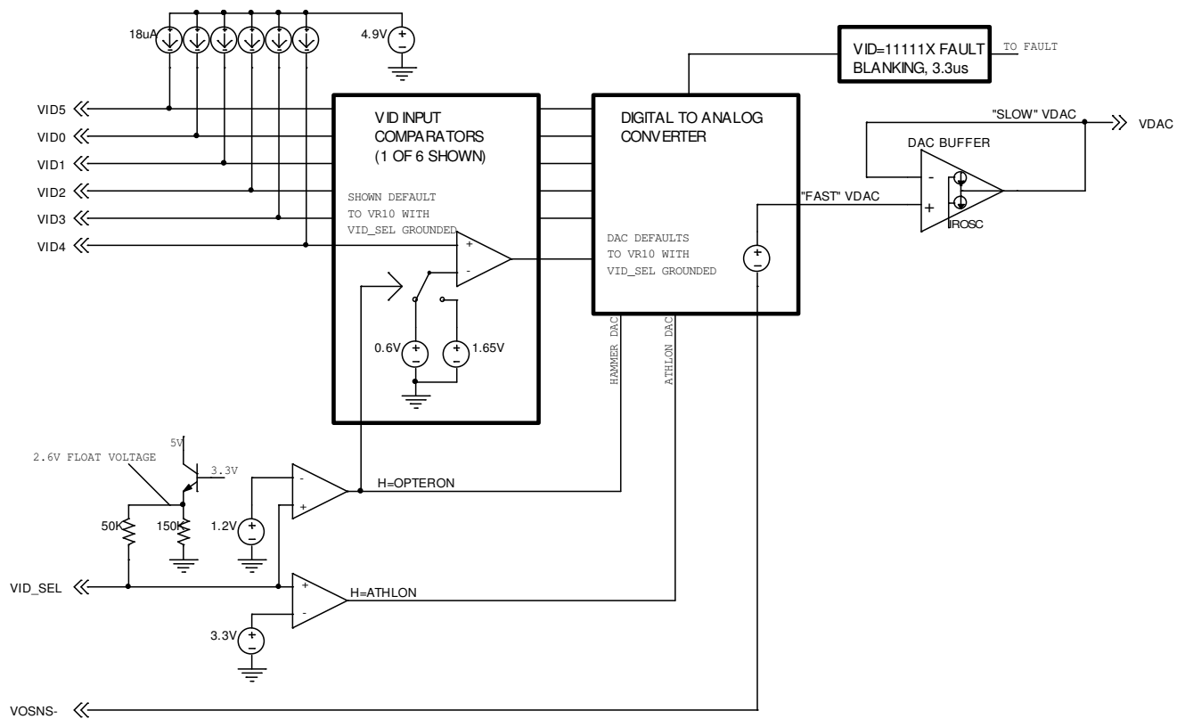
Figure 7– VID Control Block Diagram
