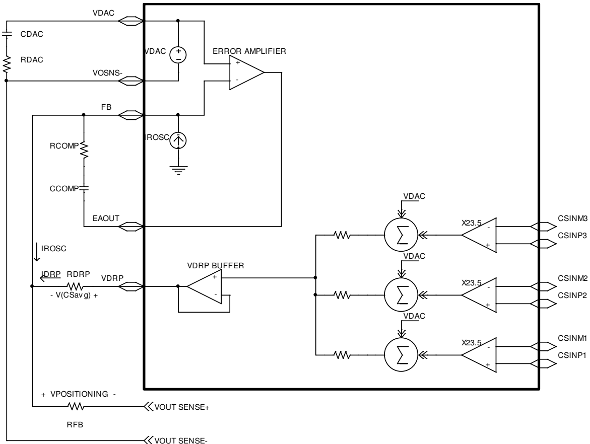
A resistor R_{FB} between FB pin and the converter output is used to create output voltage offset VO_{NLOFST} which is the difference between V_{DAC} voltage and output voltage at no load condition. An internal current source whose value is programmed by the same external resistor that programs the oscillator frequency, R_{ROSC} , pumps current I_{FB} out of the FB pin.
