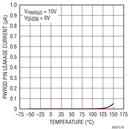
PWRGD Pin Leakage Current
