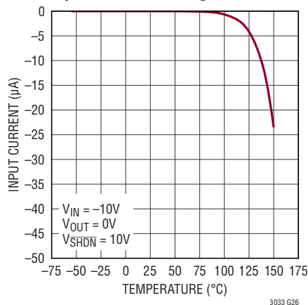
Input Reverse Leakage Current
