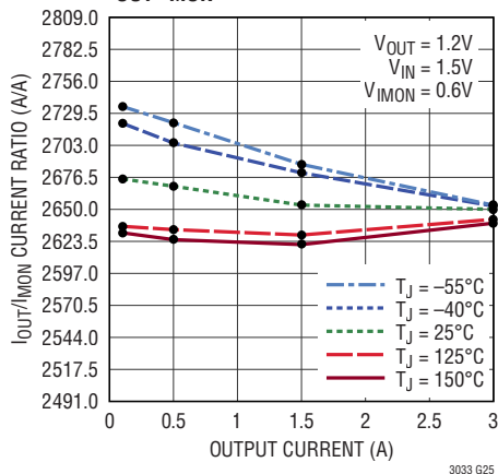
I OUT /I MON Current Ratio
