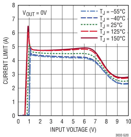
Internal Current Limit
