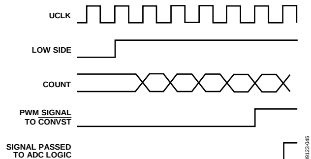
Figure 50. ADC Conversion
