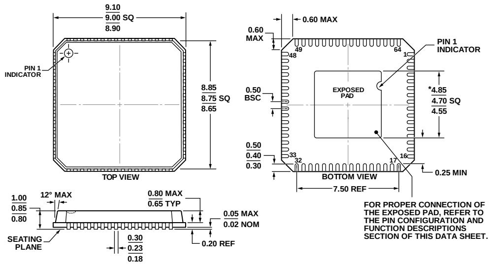
Figure 70. 64-Lead Frame Chip Scale Package [LFCSP_VQ] 9 mm x 9 mm Body, Very Thin Quad (CP-64-1)
