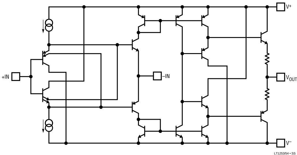
One Amplifier
