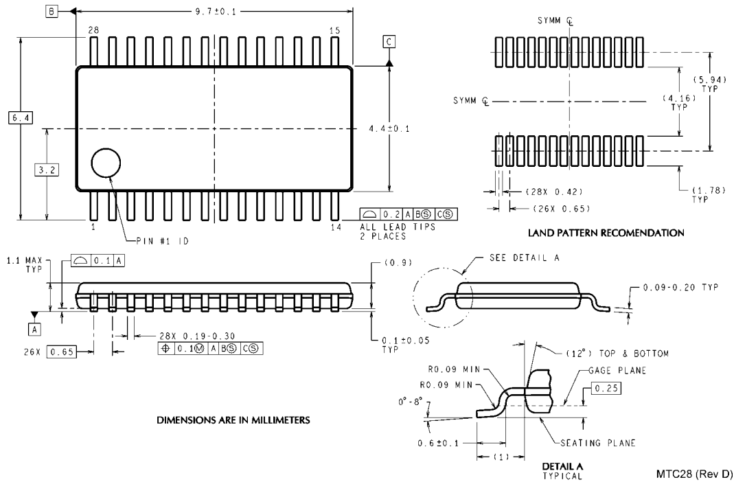
NS Package Drawing MTC28
