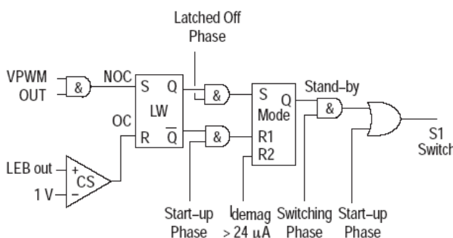
Figure 8. Transition Logic
