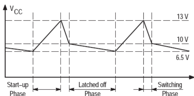
Figure 7. Hiccup Mode
