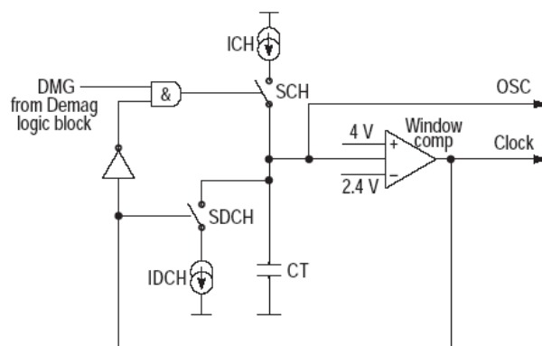
Figure 5. Oscillator Block
