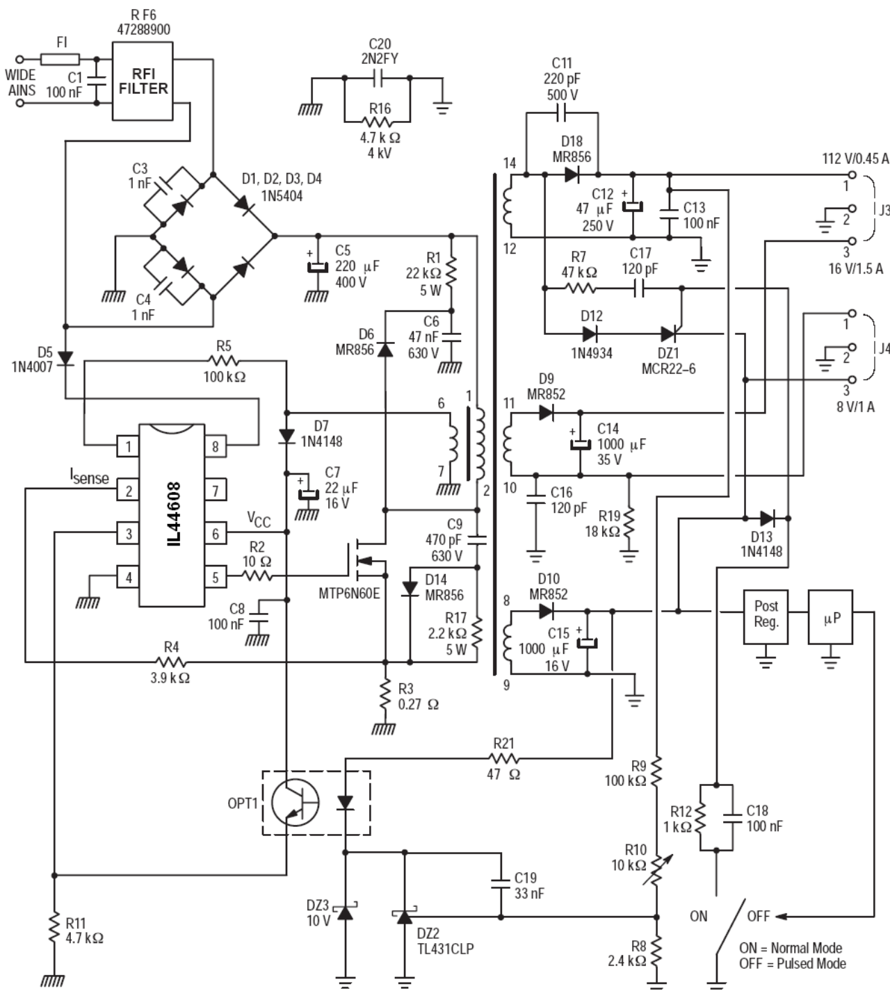
Figure 12. Typical Application
