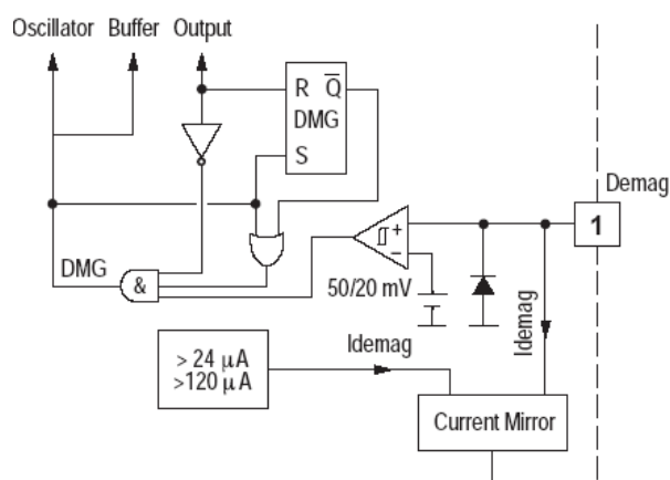
Figure 4. Demagnetization Block
