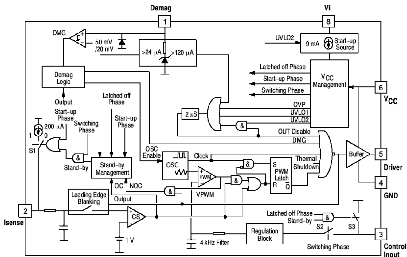
Figure 1. Representative Block Diagram
