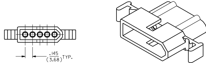
PLUG HOUSING SHOWN WITH STANDARD EARS
