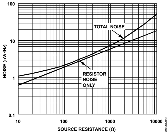
Figure 33. Noise vs. Source Resistance
