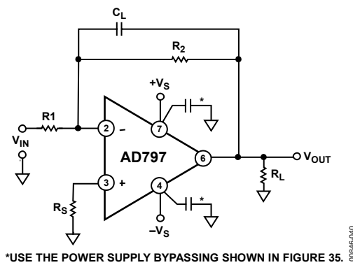
Figure 40. Inverting Amplifier Connection
