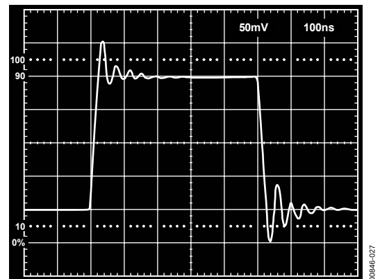
Figure 27. Follower Small-Signal Pulse Response
