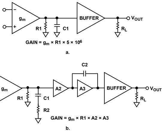
Figure 30. Model of AD797 vs. That of a Typical Three-Stage Amplifier
