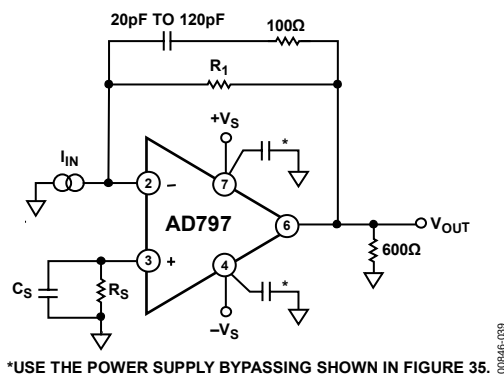
Figure 39. I-to-V Converter Connection
