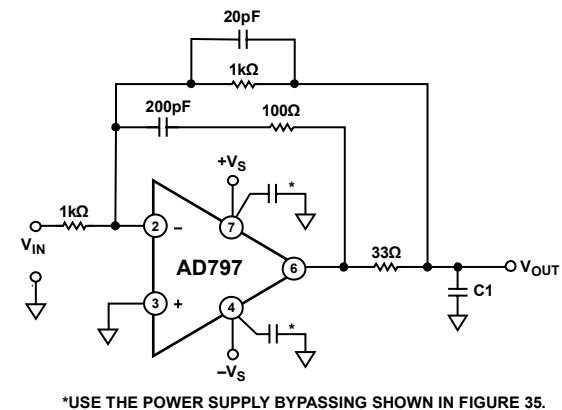
Figure 42. Recommended Circuit for Driving a High Capacitance Load
