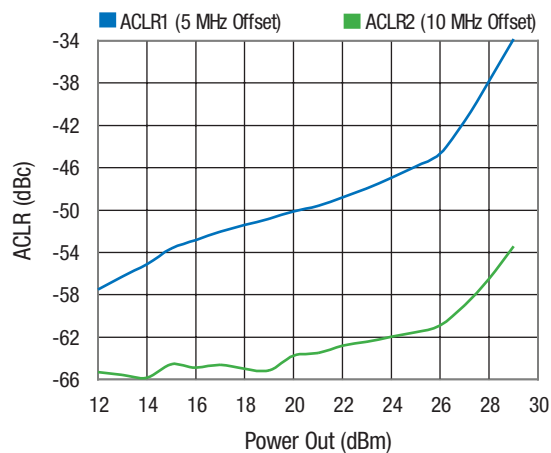
ACLR vs. Power Out WCDMA Test Tone #1; 64 DPCH \Delta F = 5 and 10 MHz
