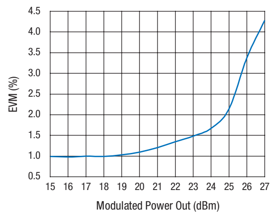
EVM vs. Modulated Power Out OFDM, 64-QAM, 54 Mbps
