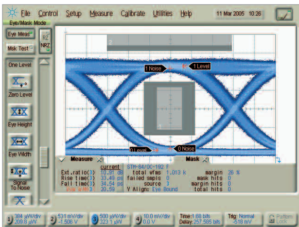
Test conditions: 9.953Gb/s 2 23 -1 PRBS NRZ data.
