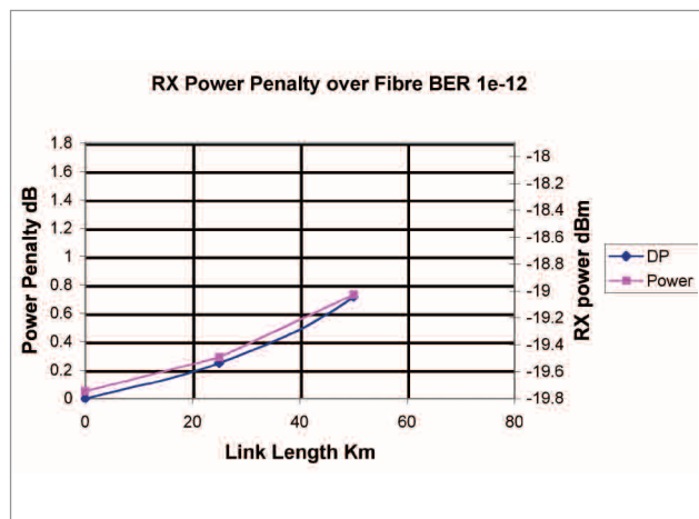
Test conditions: 9.953Gb/s 2 23 -1 PRBS NRZ data.
