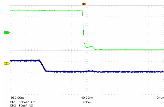
5mV input falling prop delay
