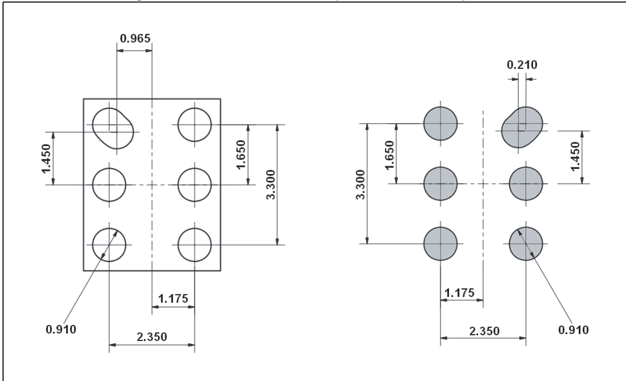
Figure 3. MP45DT02 - recommended stencil openings
