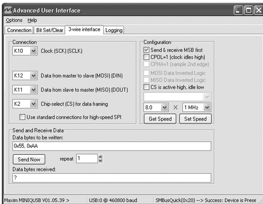
Figure 20. Advanced User Interface (3-Wire Interface Tab)
