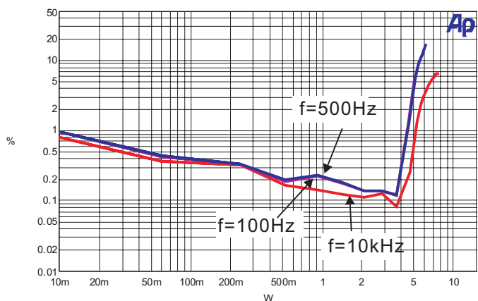
2. THD vs. Power
