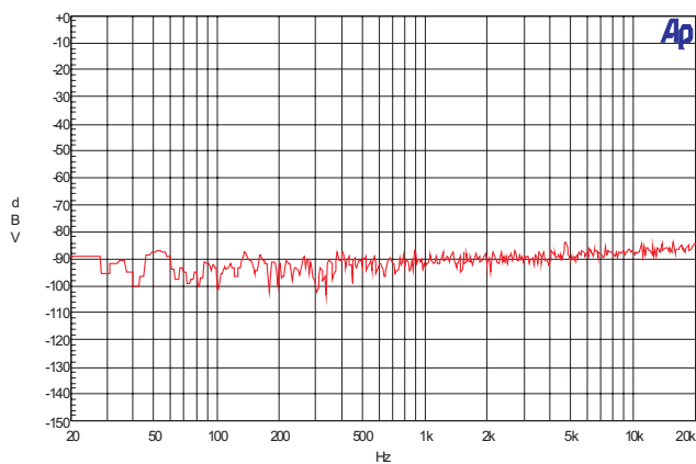
10. Noise Floor
