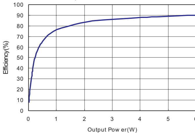
12. Efficiency vs Power
