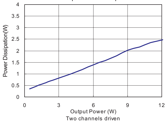
16. Power Dissipation vs. Output Power
