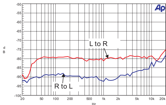
8. Crosstalk
