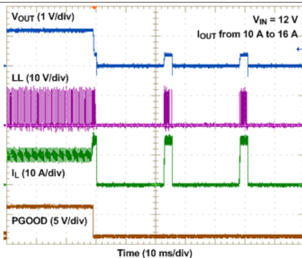
Figure 41. Overcurrent Protection
