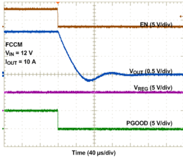
Figure 37. Shutdown
