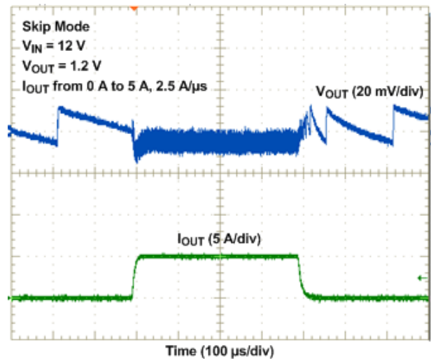
Figure 40. Skip Mode Load Transient
