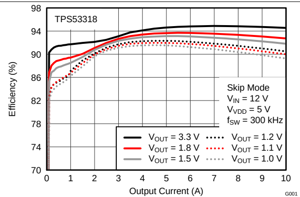
Figure 25. Efficiency vs Output Current
