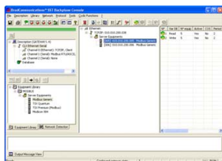
- Configuration Console -
