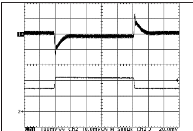
Figure 11: Output voltage response to step-change in load current (50%-75%-50% of I_{out(max)} ; dI/dt = 0.1\text{A}/\mu\text{s} ). Load cap: 15μF, 450 mΩ ESR tantalum capacitor and 1μF ceramic capacitor. Ch1: V_{out} (100mV/div), Ch2: I_{out} (5A/div).
