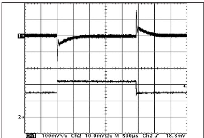
Figure 12: Output voltage response to step-change in load current (50%-75%-50% of I_{out(max)} ; dI/dt = 5\text{A}/\mu\text{s} ). Load cap: 470μF, 30 mΩ ESR tantalum capacitor and 1μF ceramic cap. Ch1: V_{out} (100mV/div), Ch2: I_{out} (5A/div).
