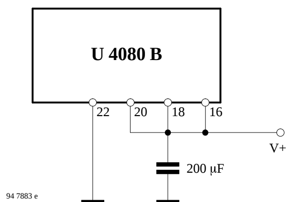
Figure 14. Regulated power supply
