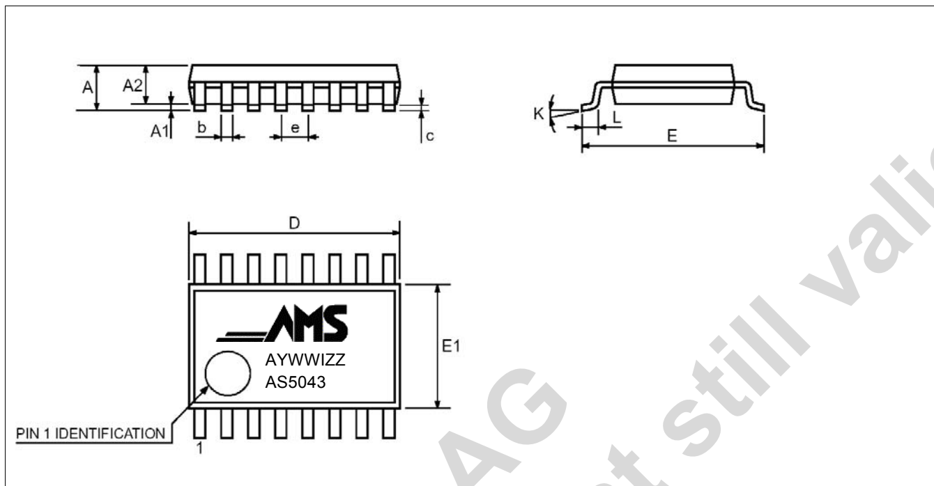
Figure 25: 16-Lead Shrink Small Outline Package SSOP-16
