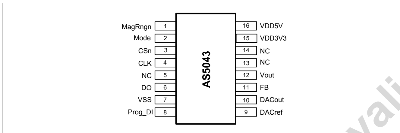
Figure 2: AS5043 Pin Configuration SSOP16
