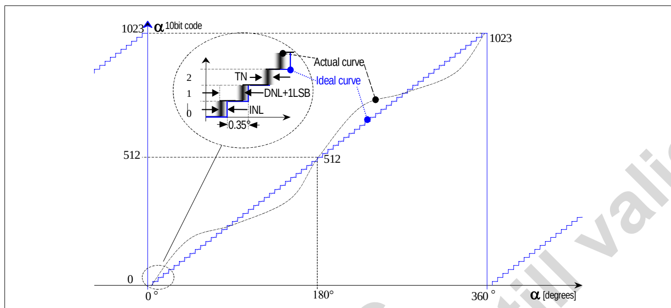
Figure 24: Integral and Differential Non-Linearity (exaggerated curve)
