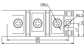
Fig. 8 - Outline Characteristics
