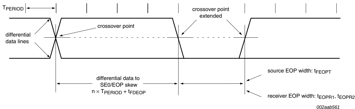
Fig 25. Differential data-to-EOP transition skew and EOP width
