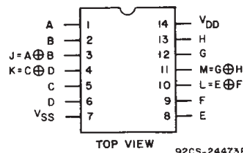
TOP VIEW 92CS-24473RI
