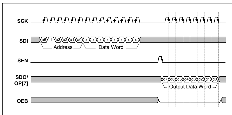
Figure 20 Serial Interface Register Read-back
